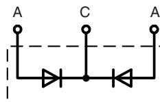
TO-264 A
