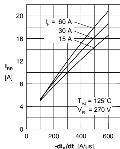
Fig. 3 Typ. reverse recovery current I_{RR} versus -di_F/dt
