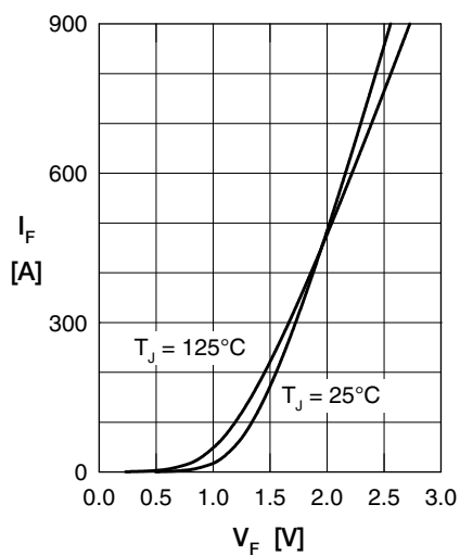
Fig. 7 Typ. forward characteristics of free wheeling diode
