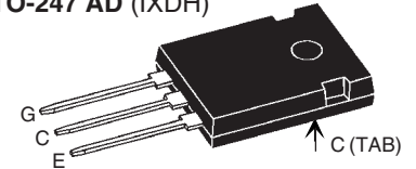
TO-247 AD (IXDH)
