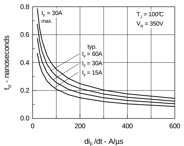
Fig.17 Reverse Recovery Time t_{rr}
