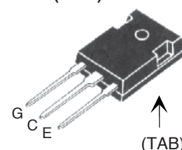
TO-247 (IXFH)
