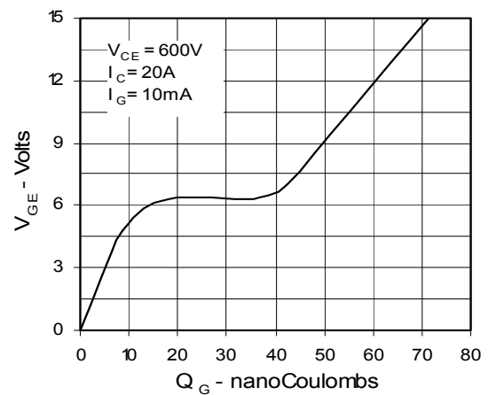
Fig. 10. Gate Charge
