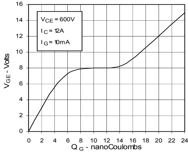
Fig. 13. Gate Charge
