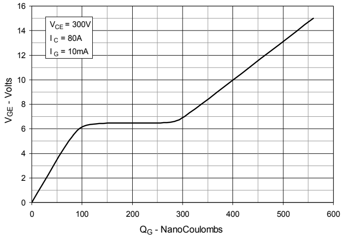
Fig. 7. Gate Charge
