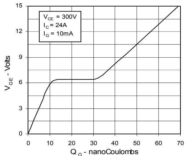
Fig. 14. Gate Charge
