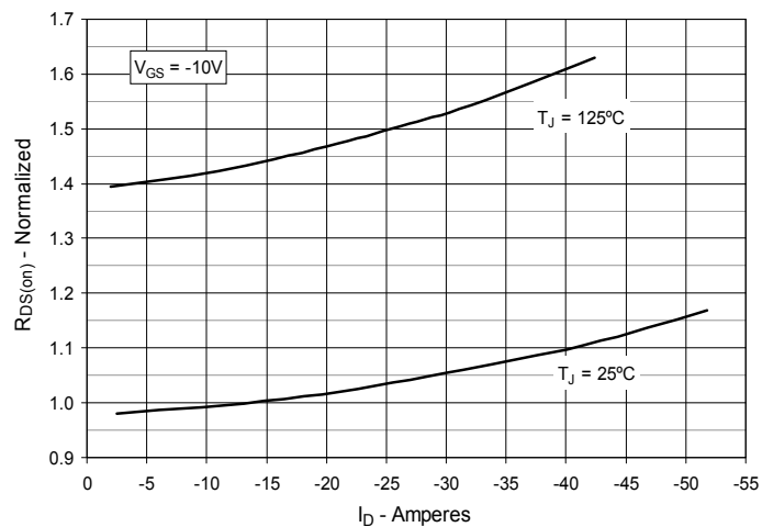
Fig. 5. R_{DS(on)} Normalized to I_D = -14\text{A} vs. Drain Current
