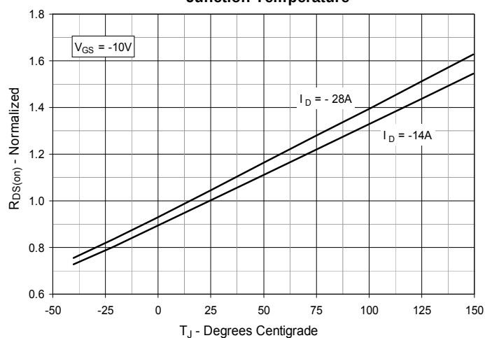
Fig. 4. R_{DS(on)} Normalized to I_D = -14\text{A} vs. Junction Temperature
