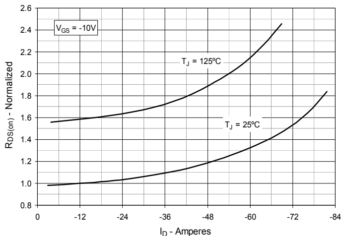
Fig. 5. R_{DS(on)} Normalized to I_D = -12\text{A} vs. Drain Current
