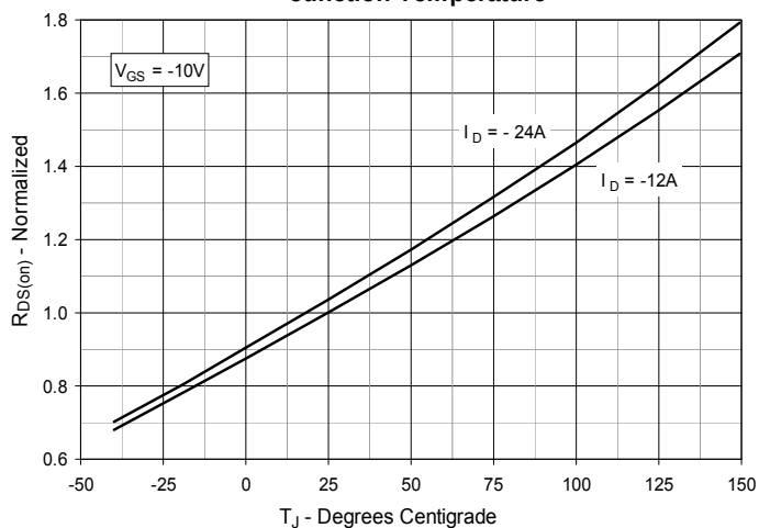
Fig. 4. R_{DS(on)} Normalized to I_D = -12\text{A} vs. Junction Temperature
