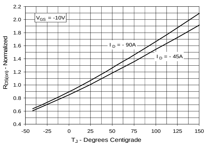
Fig. 4. R_{DS(on)} Normalized to I_D = -45\text{A} vs. Junction Temperature
