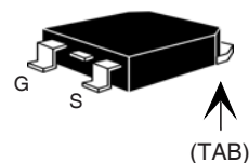
TO-268 (IXTT)
