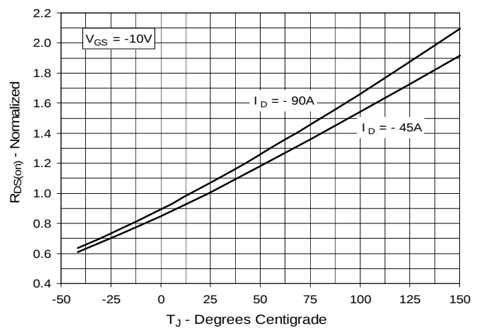
Fig. 4. R_{DS(on)} Normalized to I_D = -45\text{A} vs. Junction Temperature
