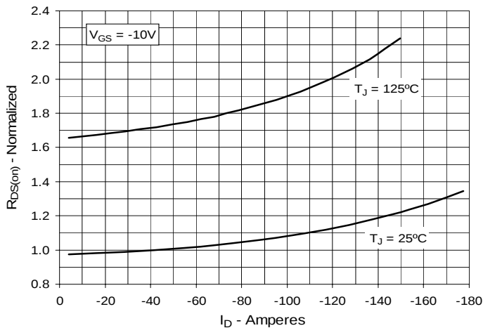
Fig. 5. R_{DS(on)} Normalized to I_D = -45\text{A} vs. Drain Current
