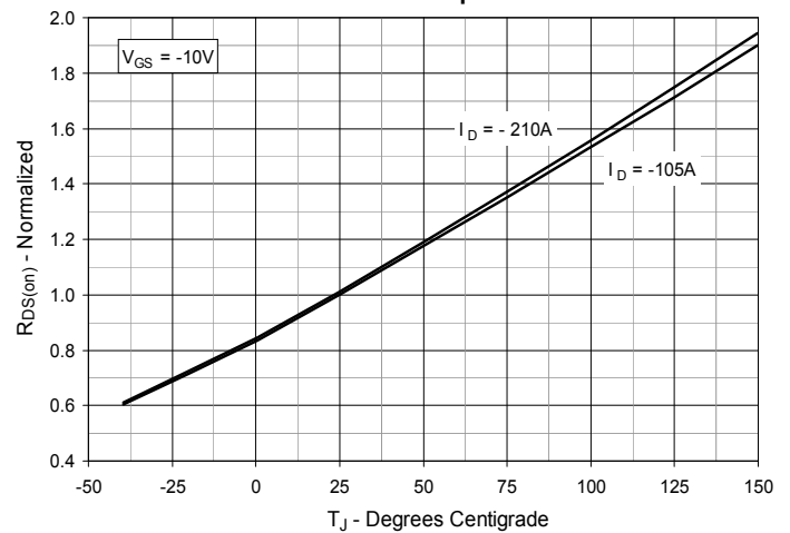
Fig. 4. R_{DS(on)} Normalized to I_D = -105\text{A} vs. Junction Temperature
