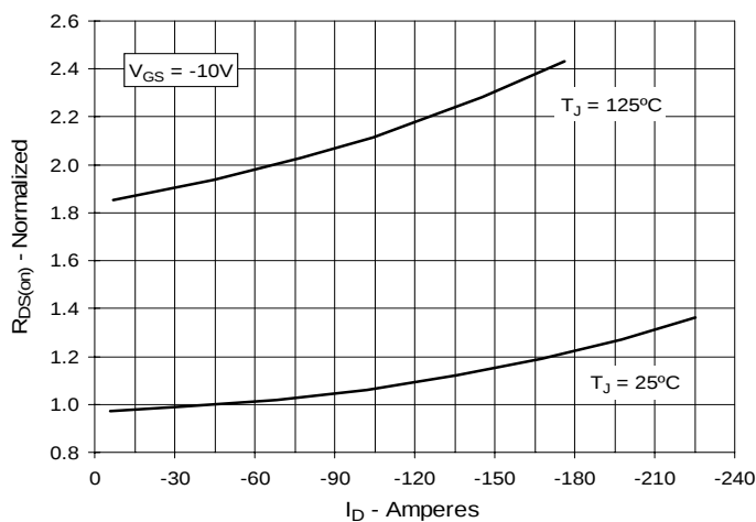
Fig. 5. R_{DS(on)} Normalized to I_D = -45A vs. Drain Current
