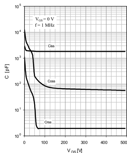
Fig. 9 Typ. capacitances
