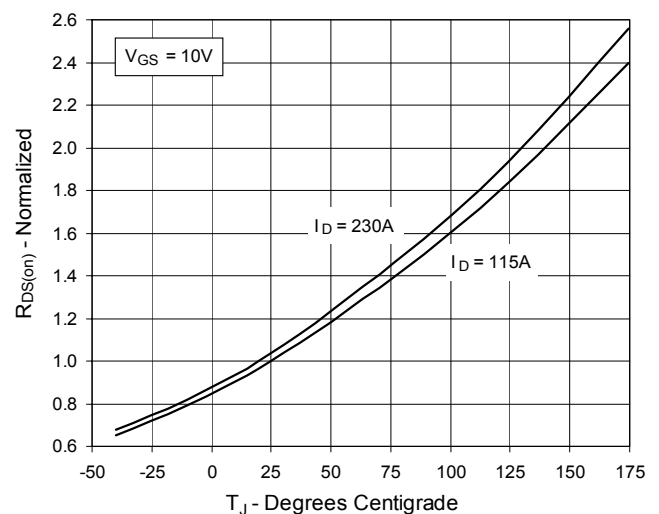
Fig. 4. R_{DS(on)} Normalized to I_D = 115\text{A} Value vs. Junction Temperature
