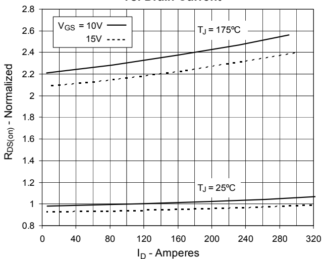
Fig. 5. R_{DS(on)} Normalized to I_D = 115\text{A} Value vs. Drain Current
