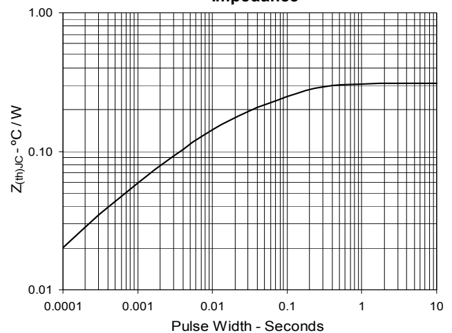
Fig. 19. Maximum Transient Thermal Impedance
