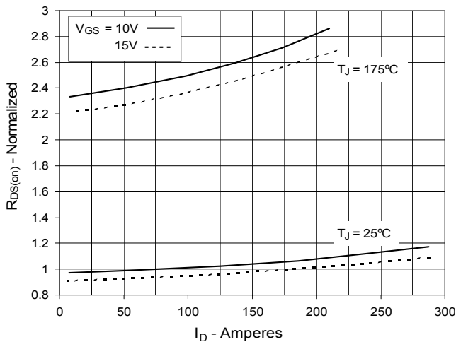
Fig. 5. R_{DS(on)} Normalized to I_D = 76A Value vs. Drain Current
