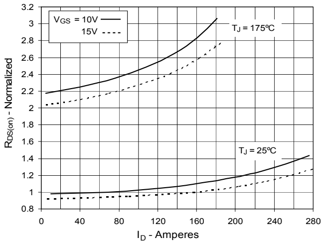
Fig. 5. R_{DS(on)} Normalized to I_D = 44A Value vs. Drain Current
