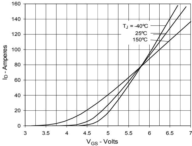
Fig. 7. Input Admittance
