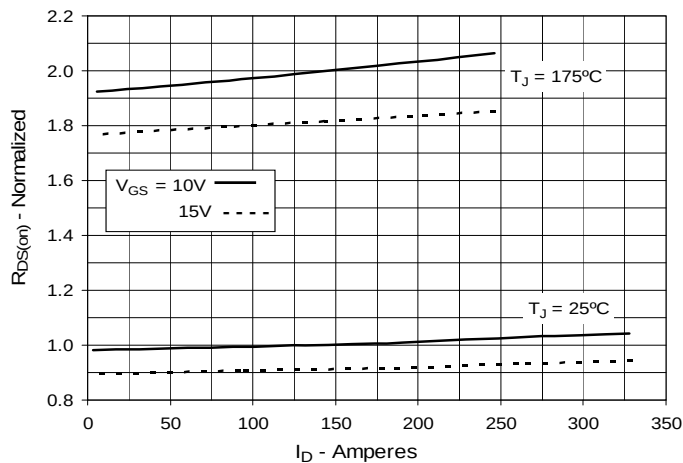
Fig. 5. R_{DS(on)} Normalized to I_D = 140A Value vs. Drain Current
