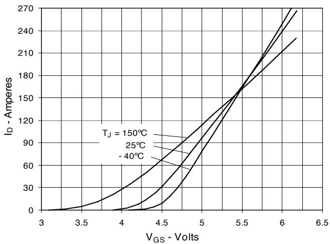
Fig. 7. Input Admittance
