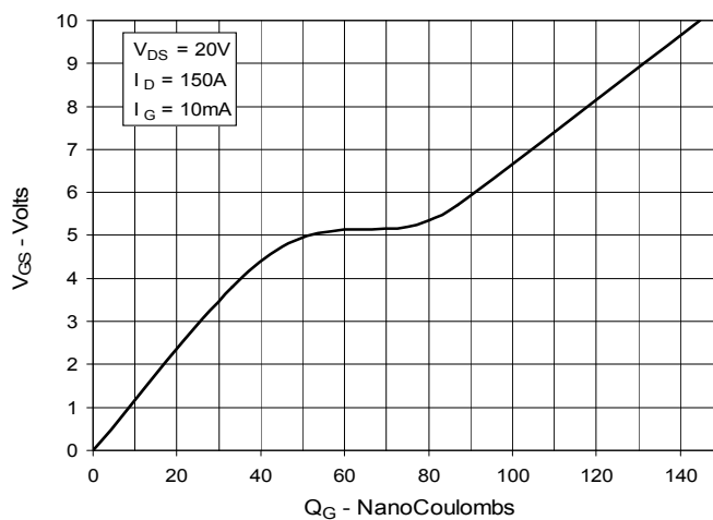
Fig. 10. Gate Charge
