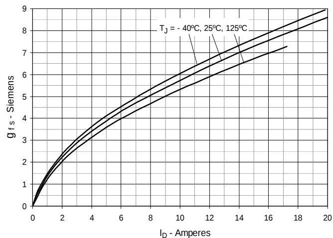
Fig. 8. Transconductance
