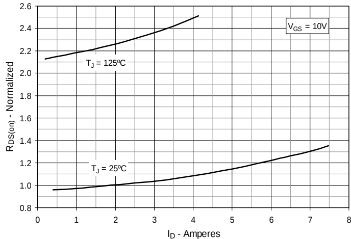
Fig. 5. R_{DS(on)} Normalized to I_D = 2A Value vs. Drain Current
