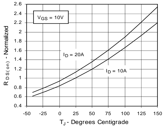
Fig. 4. R_{DS(on)} Normalized to I_D = 10A Value vs. Junction Temperature
