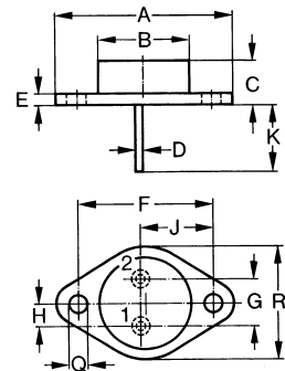
TO-204 AE (IXFM) Outline
