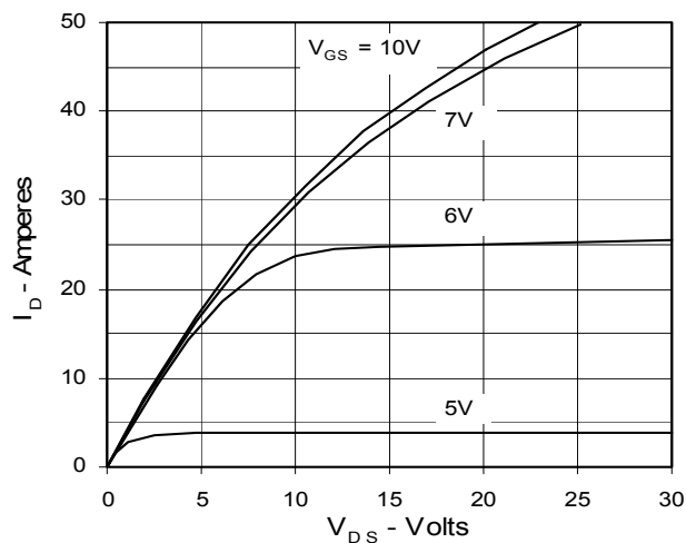
Fig. 2. Extended Output Characteristics @ 25 deg. C
