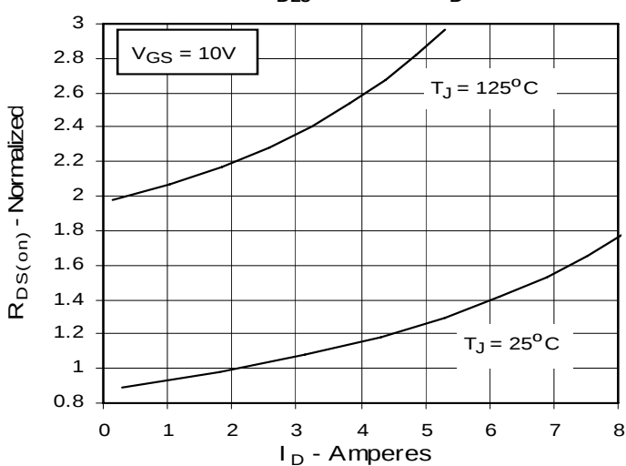
Fig. 5. R_{DS(on)} Normalized to 0.5 I_{D25} Value vs. I_D
