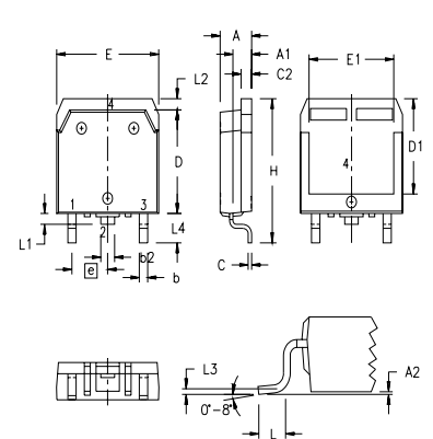
TO-268 (IXTT) Outline
