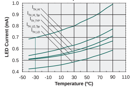
Typical LED Logic Threshold Current vs. Temperature
