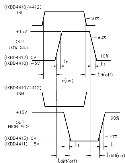
Fig. 1b: Output signal waveform
