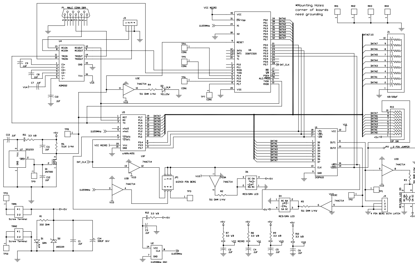
Figure 7 - EVDP610 Schematic
