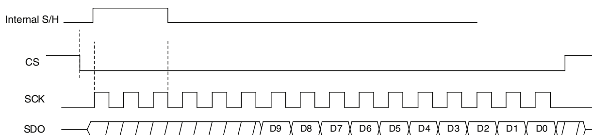
Figure 1. Serial Timing Diagram
