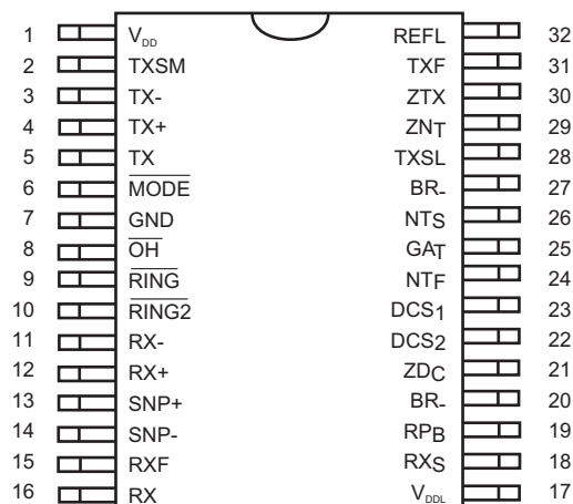
Figure 2. Pinout
