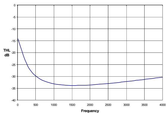
Figure 11. Transhybrid Loss
