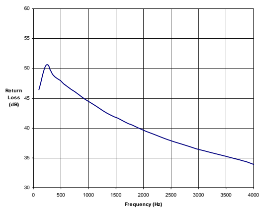
Figure 12. Return Loss
