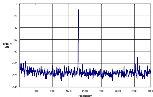
Figure 10. Transmit THD on Tip and Ring
