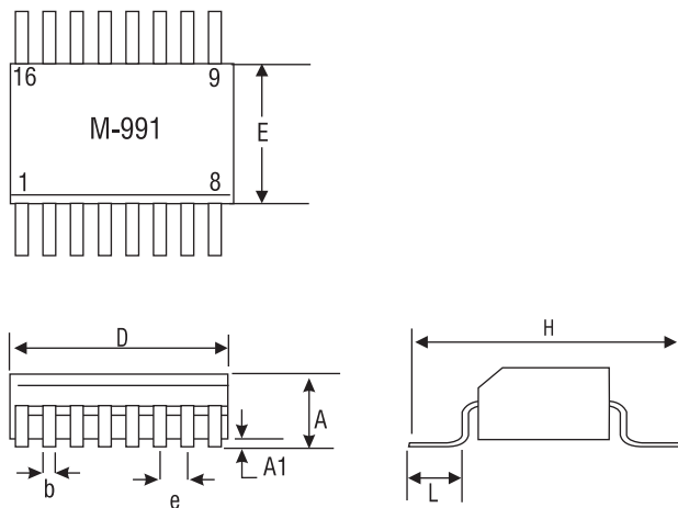
16-Pin SOIC
