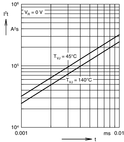
Fig. 4 I^2t versus time (1-10 ms)
