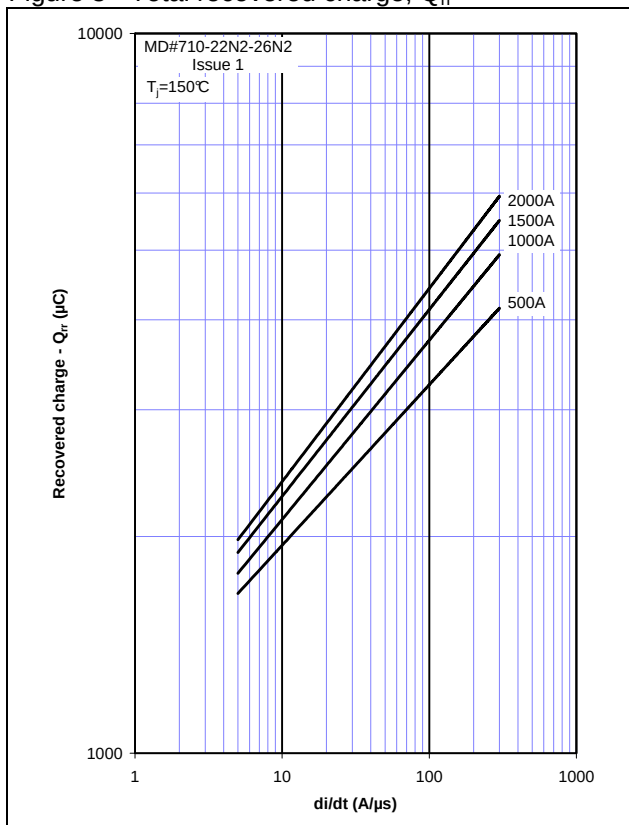
Figure 3 - Total recovered charge, Q_{rr}
