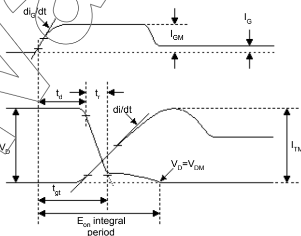
Diagram 9, Turn-on wave-diagrams.
