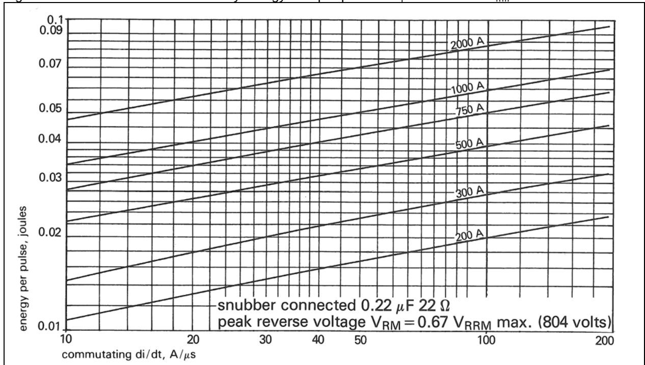
Figure 15 - Maximum reverse recovery energy loss per pulse at T_j = 125^\circ\text{C} and V_{rm} = 804 volts
