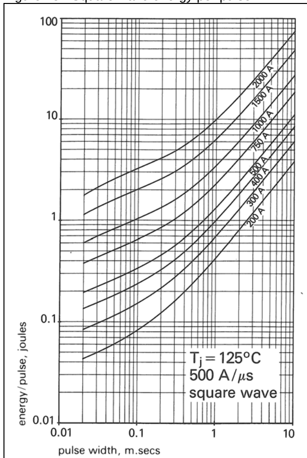
Figure 15 – Maximum reverse recovery energy loss per pulse at T_j = 125^\circ\text{C} and V_{rm} = 804 volts
