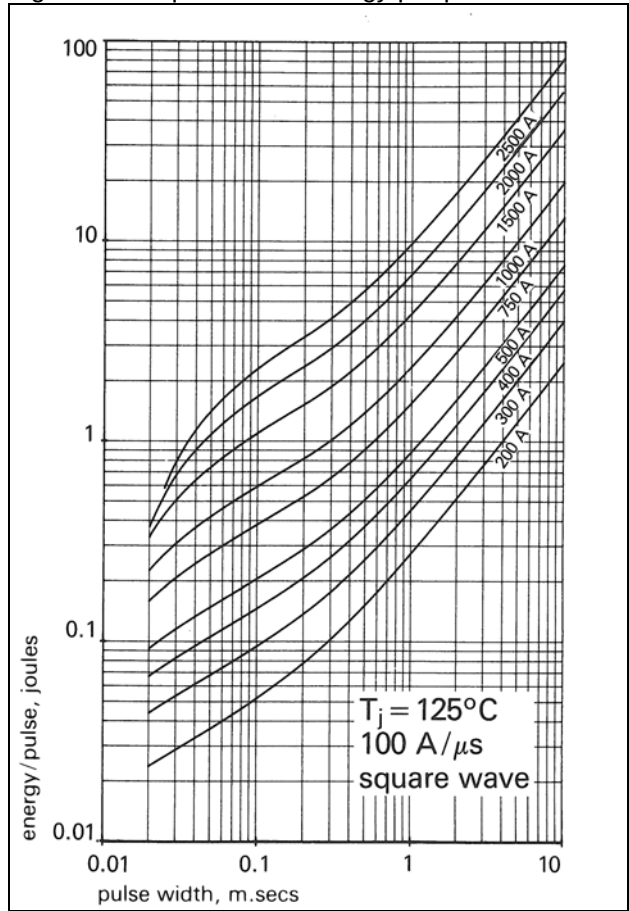
Figure 15 – Maximum reverse recovery energy loss per pulse at T_j = 125^\circ\text{C} and V_{rm} = 536 volts
