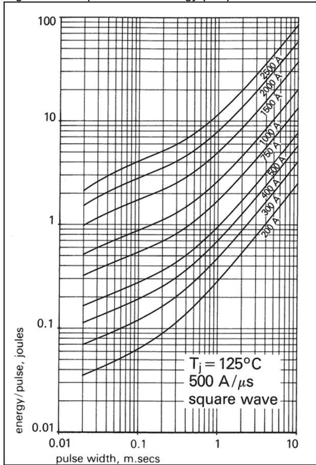
Figure 15 – Maximum reverse recovery energy loss per pulse at T_j = 125^\circ\text{C} and V_{rm} = 536 volts
