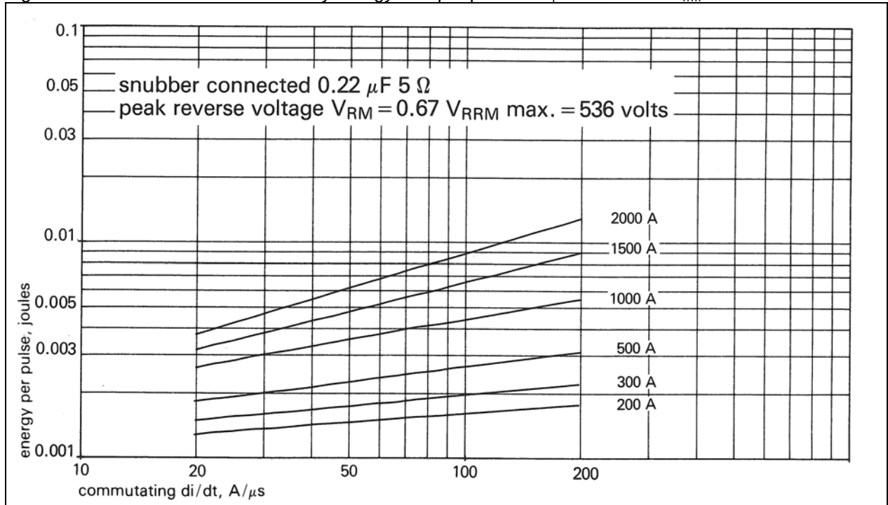
Figure 15 - Maximum reverse recovery energy loss per pulse at T_j = 125^\circ\text{C} and V_{rm} = 536\text{ volts}
