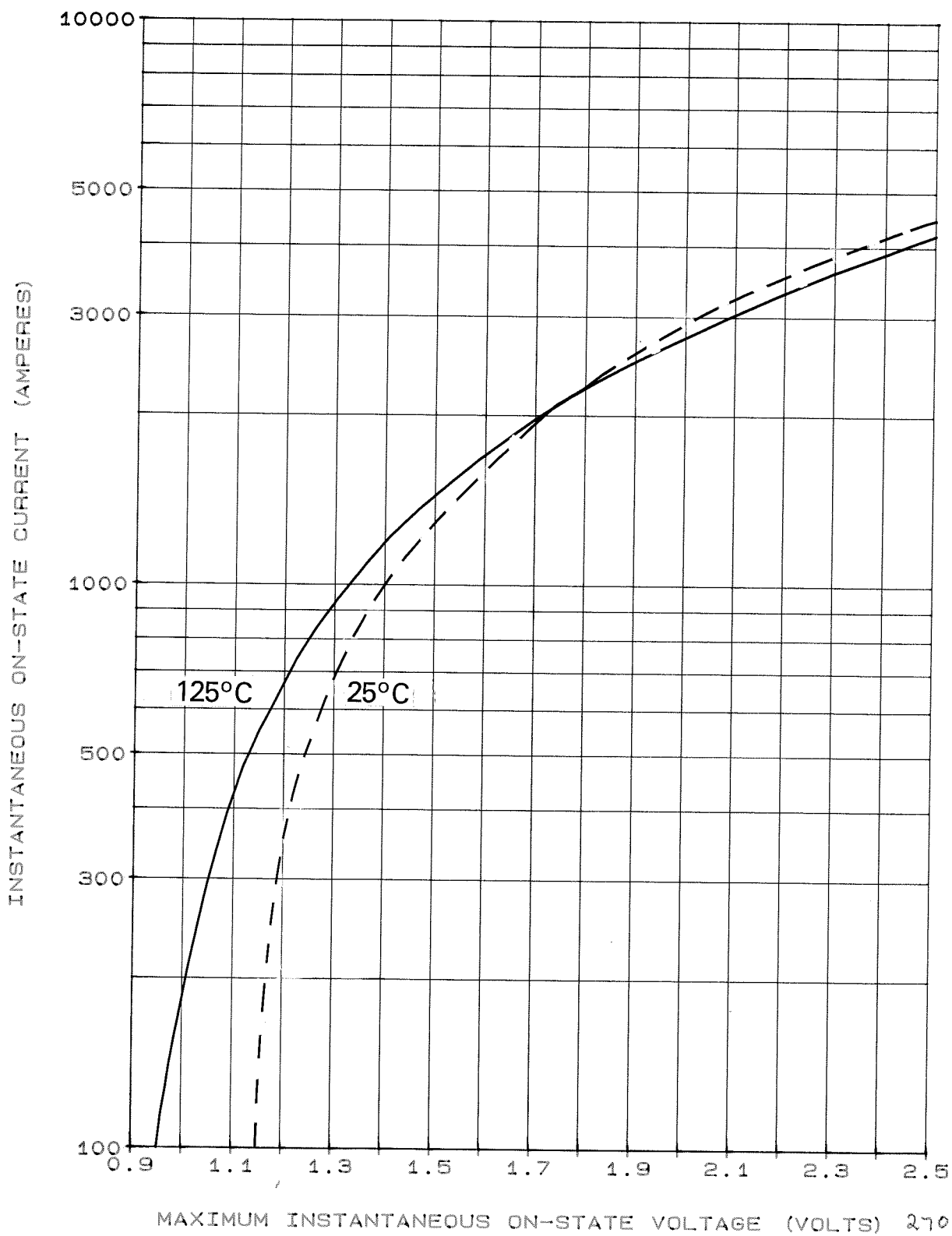
ON-STATE CHARACTERISTIC OF LIMIT DEVICE
