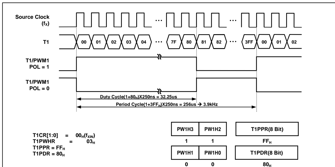
Figure 4.14 PWM Mode
