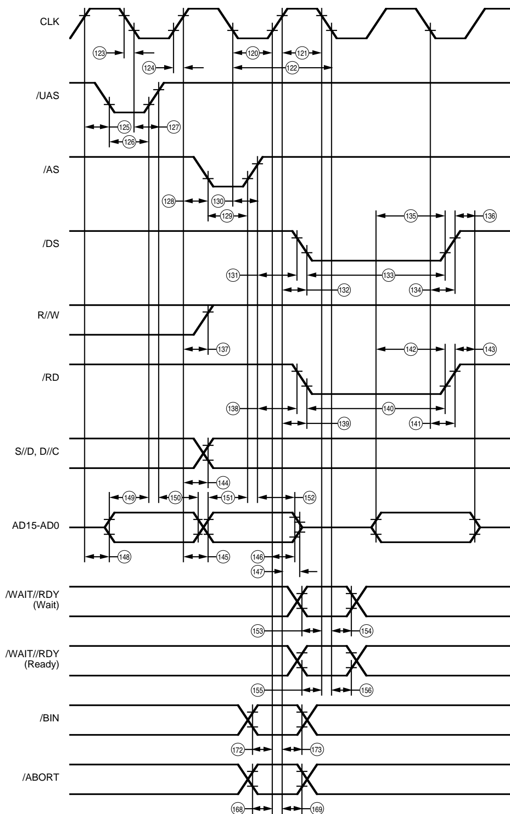
Figure 102. Memory Read
