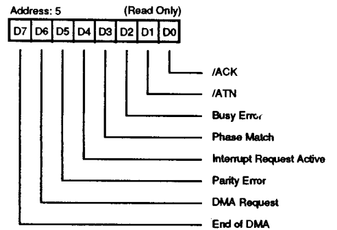
Figure 32. Bus and Status Register
