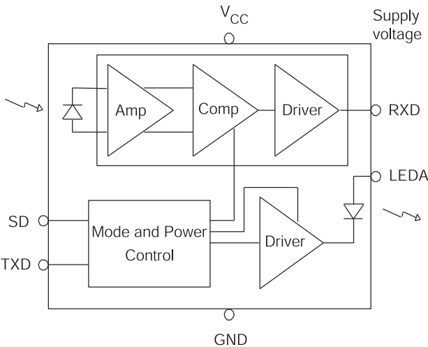
Figure 1. Slim SIR Transceiver Block Diagram
