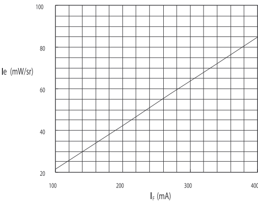
Figure 3. I_F - I_e Characteristics (0°)
