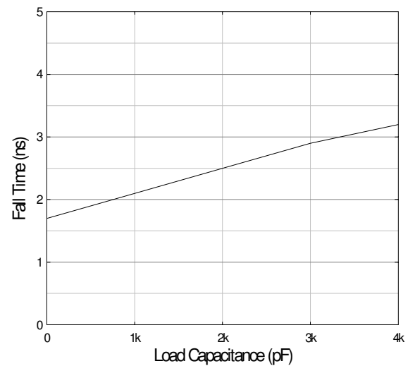
Fig. 4 Fall Time vs. Load Capacitance V_{CC} = 15V , V_{OH} = 12V To 2V
